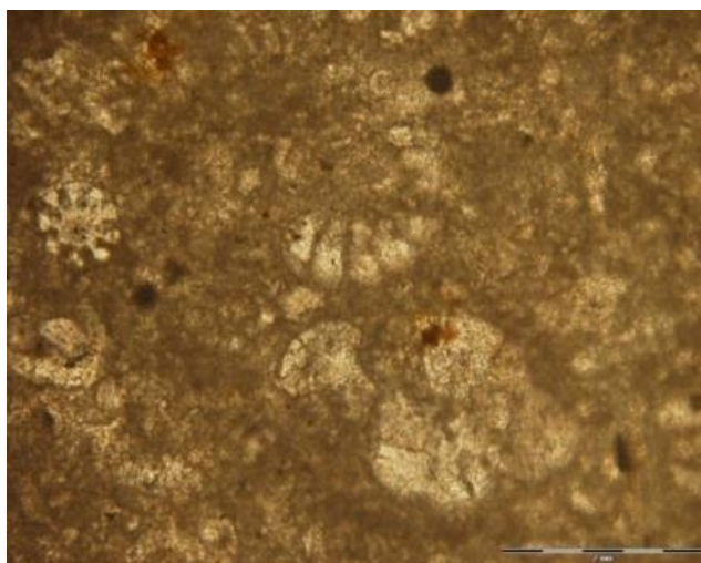
شکل ۷. Echinoid Bioclast Wackestone- packestone: Sample no. 39
